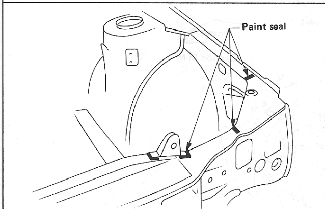
Detail C
