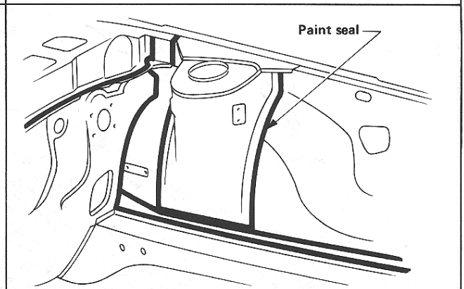
Detail D
